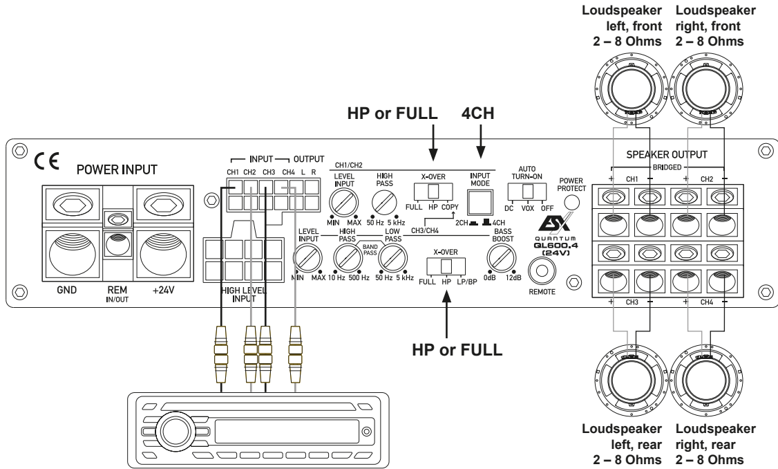
Connect stereo RCA outputs (FL/FR & RL/RR) of the head unit with INPUT CH1 / CH2 and CH3 / CH4 of the amplifier
